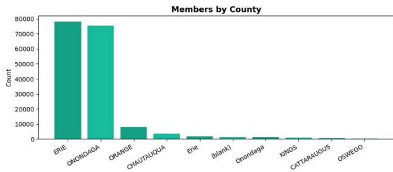
County Distribution
