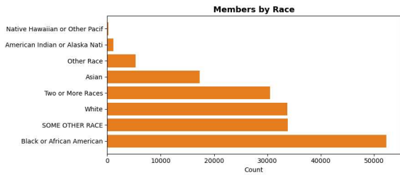
Race Distribution
