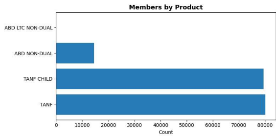
Product Distribution
