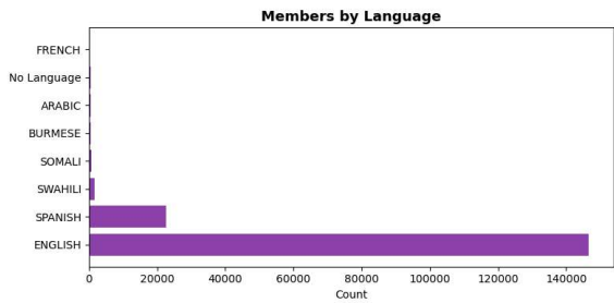
Language Distribution
